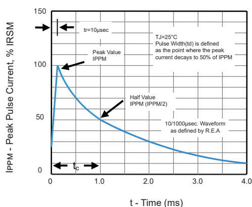
Figure 3 - Pulse Waveform
