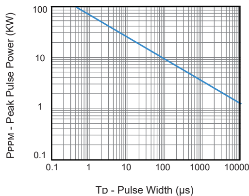
Figure 3 - Peak Pulse Power Rating Curve
