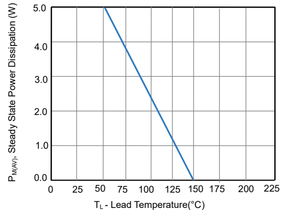
Figure 4 - Steady State Power Derating Current
