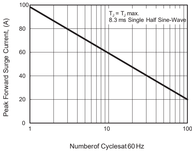
Figure 5 - Maximum Non-Repetitive Surge Current
