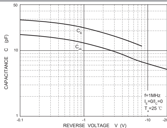
Fig. 6 C_{ob}/C_{ib} - V_{CB}/V_{EB}
