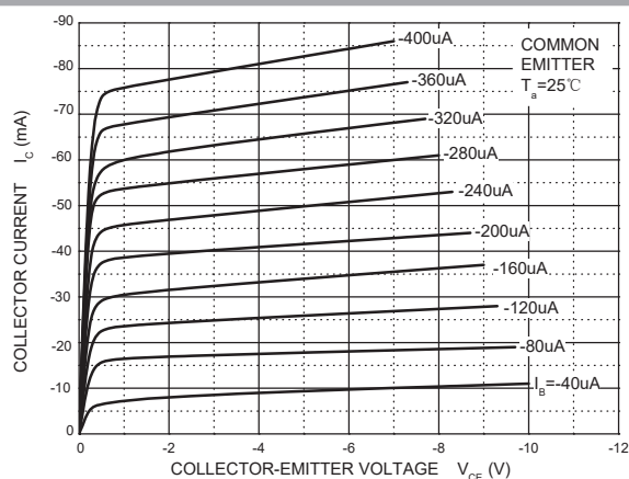
Fig. 1 Static Characteristic
