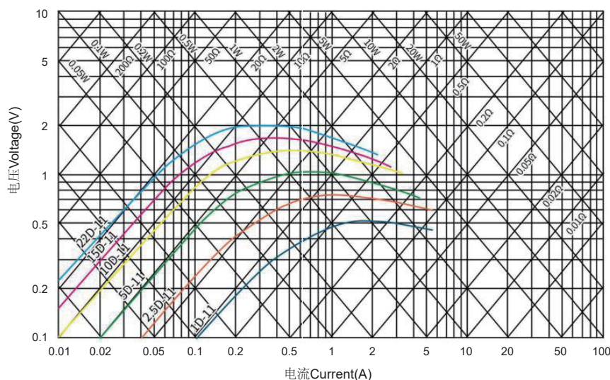
电压-电流曲线 Voltage-Current Curve
